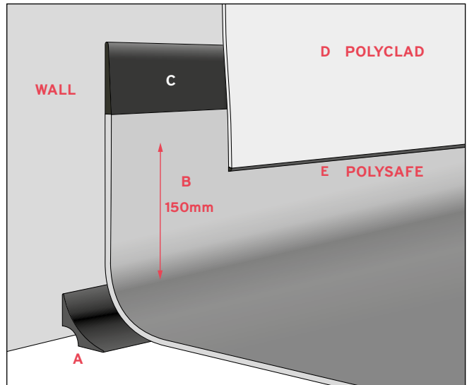
Figure 2 Overlap installation method
